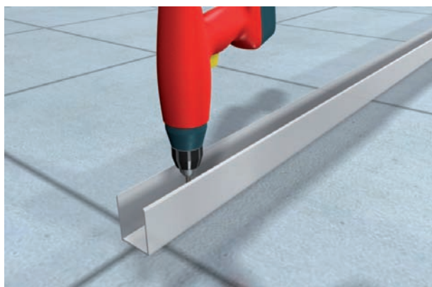
■ ASSEMBLING THE FLOOR U-EXTRUSION
