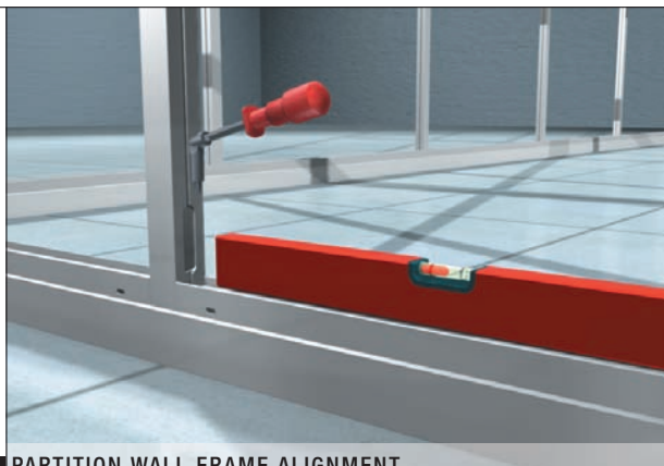
■ PARTITION WALL FRAME ALIGNMENT
