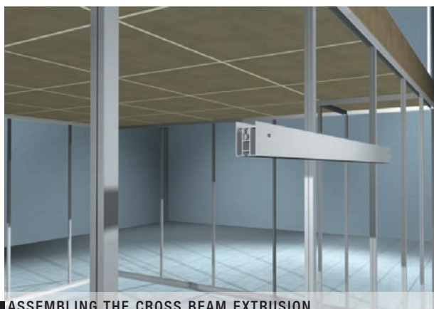
■ ASSEMBLING THE CROSS BEAM EXTRUSION
