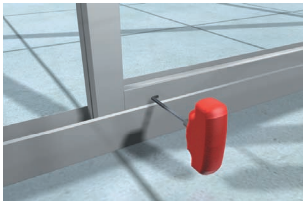
■ CONNECTING THE FLOOR BEAM WITH THE UPRIGHTS
